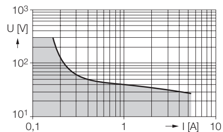
Load limit curve
