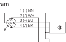
F146 - Wire-break monitoring wiring diagram
