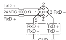
F130 - Connection - RS485 devices
