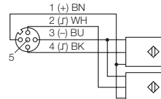
F144 - Wiring diagram
